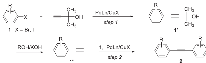
Scheme 3. Synthesis of diarylated internal alkynes from the reaction of aryl halides with 2-methyl-3-butyn-2-ol.
